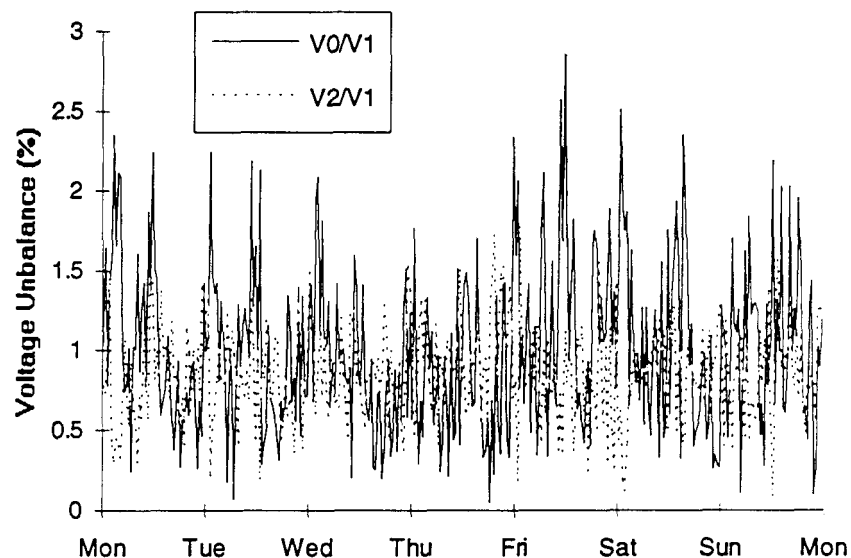
Figure 9—Imbalance trend for a residential feeder
